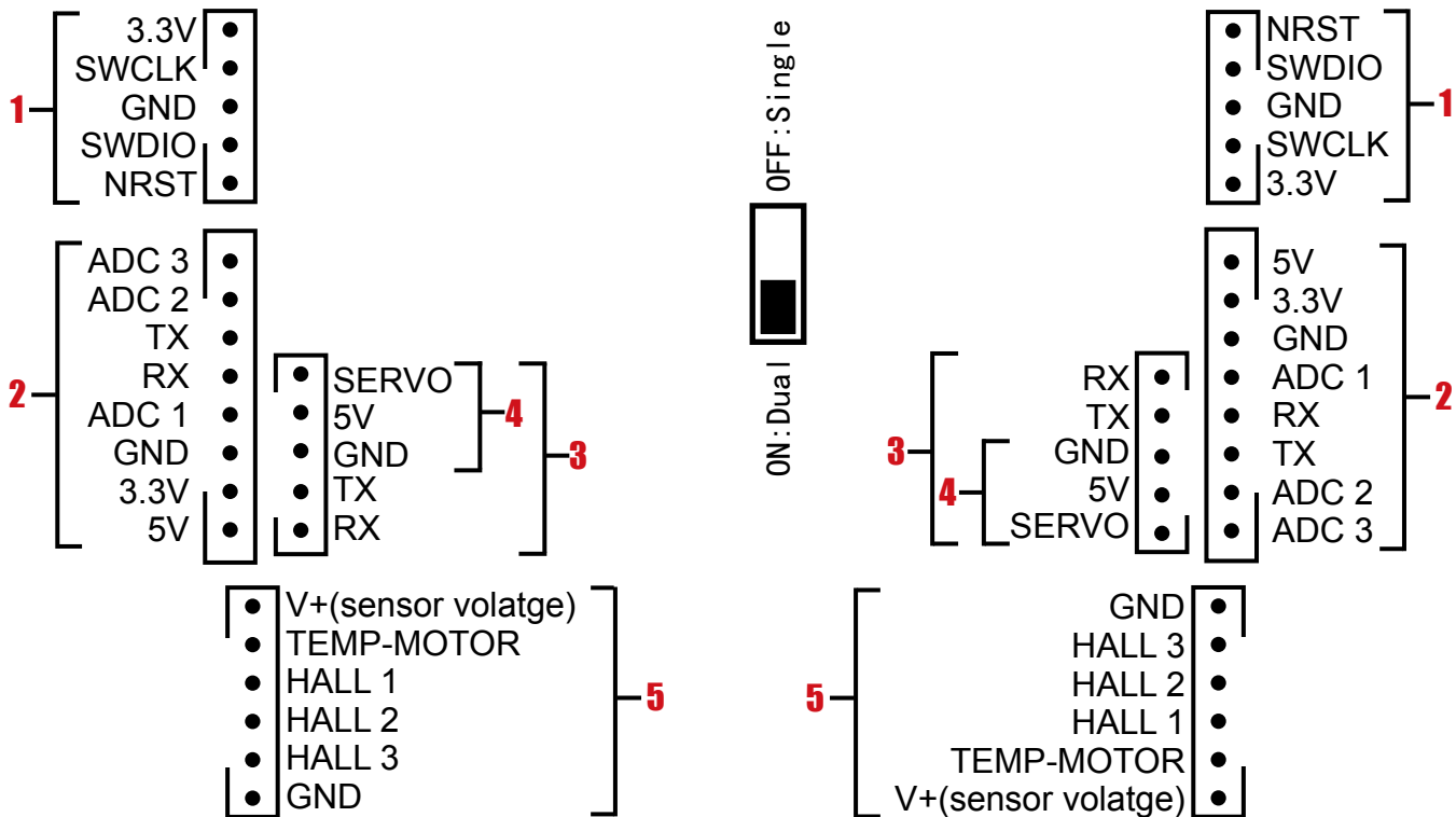
1.SWD 2.COMM 3.RECEIVER 4.PPM 5.SENSE
